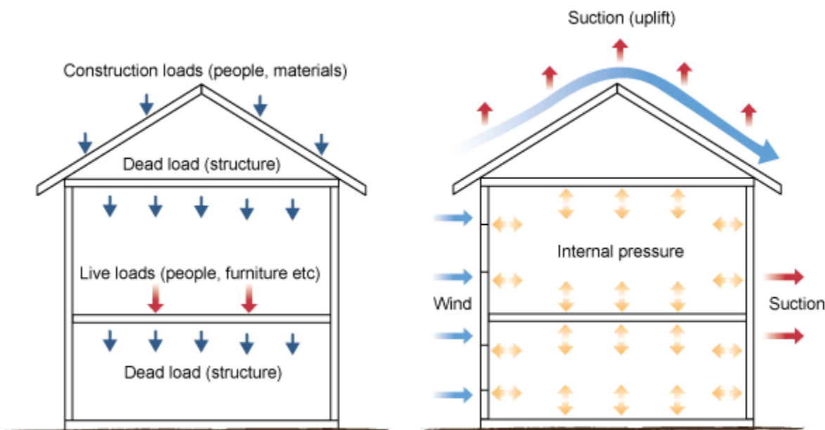
Figure 42. Illustration of loads created by wind pressure showing how internal and external forces work together to put a strain on the windward and leeward sides of a structure.
