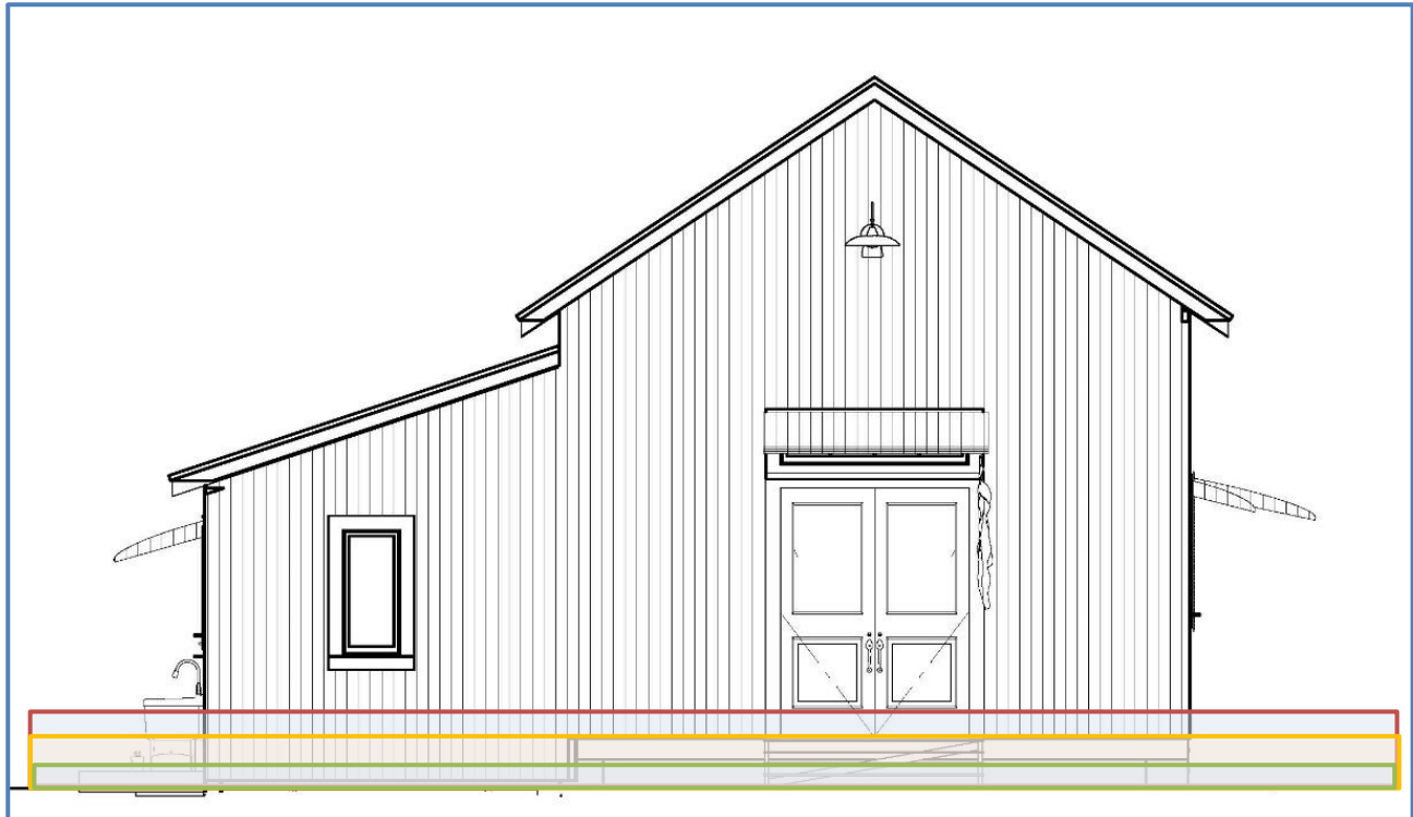
Figure 31. The National Register building, “Meres Packing House” (see Figure 12) showing the general elevation of flood waters at one (green), two (orange) and three (red) feet above grade. This building has corrugated metal walls, a pier-supported foundation, and wood floor without a sub-floor. The ground elevation at this building entrance is less than three (3) feet above sea level.
